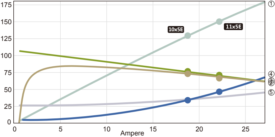
Motor Characteristics
